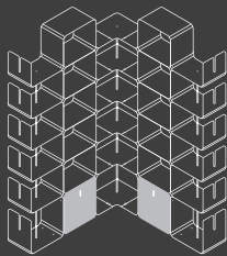
J UNBL-56D2 L1372-1372 x H2232mm
